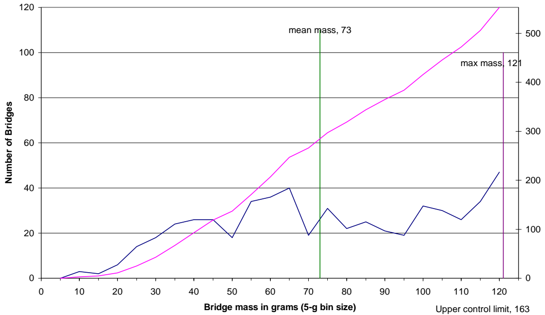
Histogram of bridge mass in-specification bridges, toothpick category, 1992 through 2004
