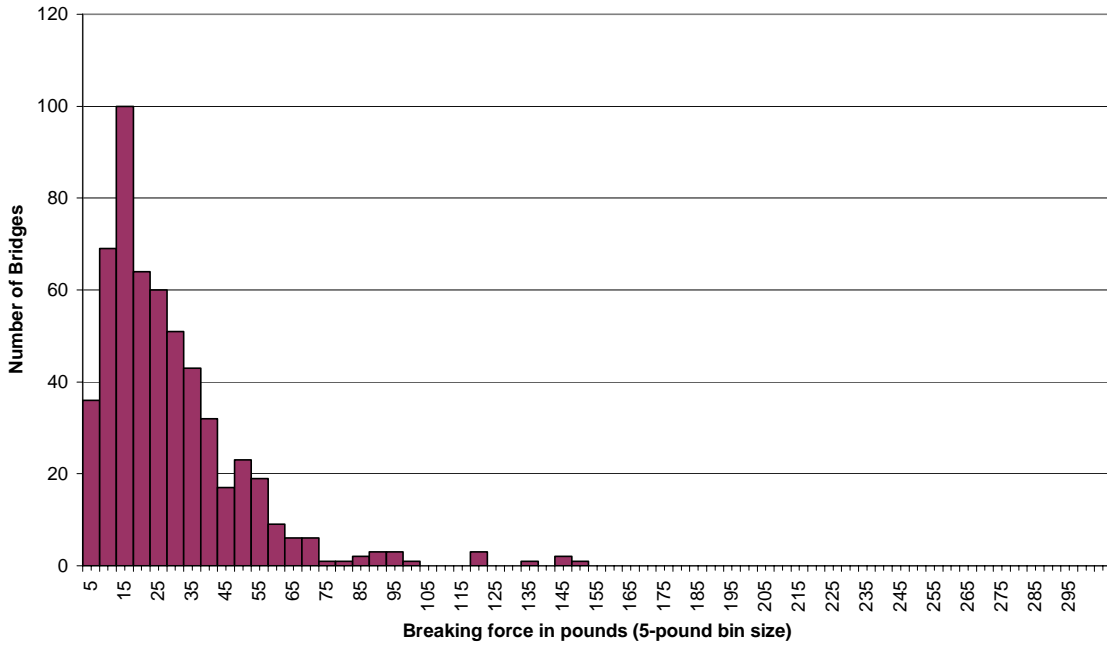
Histogram of breaking force in-specification bridges, toothpick category, 1992 through 2004
