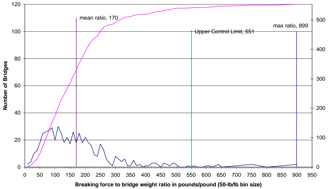
Histogram of breaking force to bridge weight ratio in-specification bridges, toothpick category, 1992 through 2004
